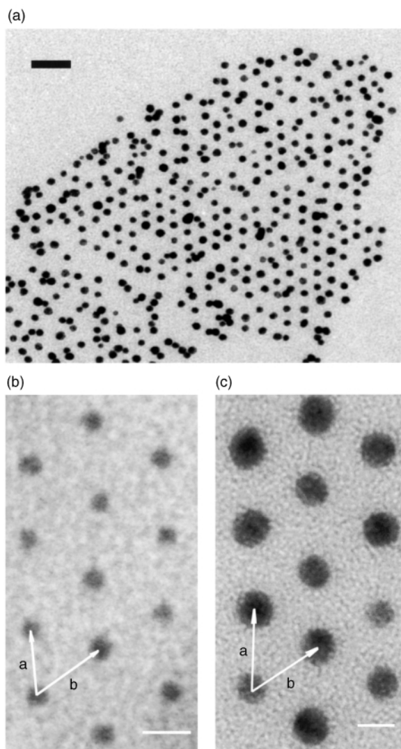
Fig. 8 TEM micrographs of S-layer templated gold nanoparticle superlattices. (a) Low magnification image showing single crystal domain with defects, scale bar = 40 nm. (b) and (c) 2-D hexagonal arrays of 5 and 10 nm gold nanoparticles with interparticle contact distances of ca. 12 and 7 nm, respectively. Vectors a and b show an average centre-to-centre spacing of 18 nm in both cases. Scale bars = 10 nm.
