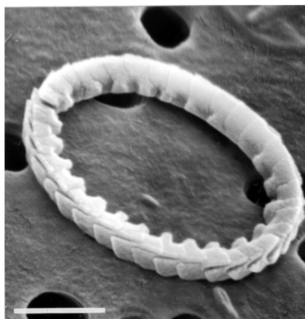
Fig. 3 SEM image of the initial stage of coccolith biomineralization in the alga Emiliana huxleyi . Each calcite crystal in the interlocked ring is crystallographically aligned and spatially discrete. Scale bar = 0.5 \mu\text{m} .
